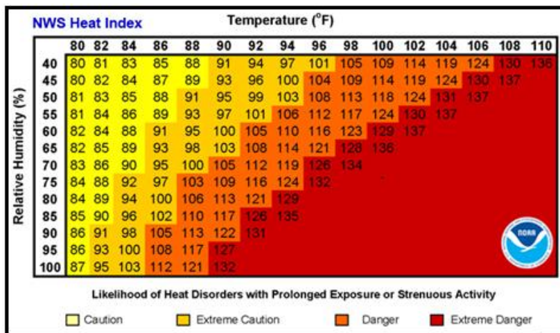
Chart 3: Heat Index
