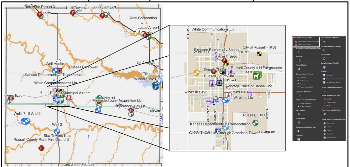
Map 80: Russell County Critical Infrastructure in Floodplains
