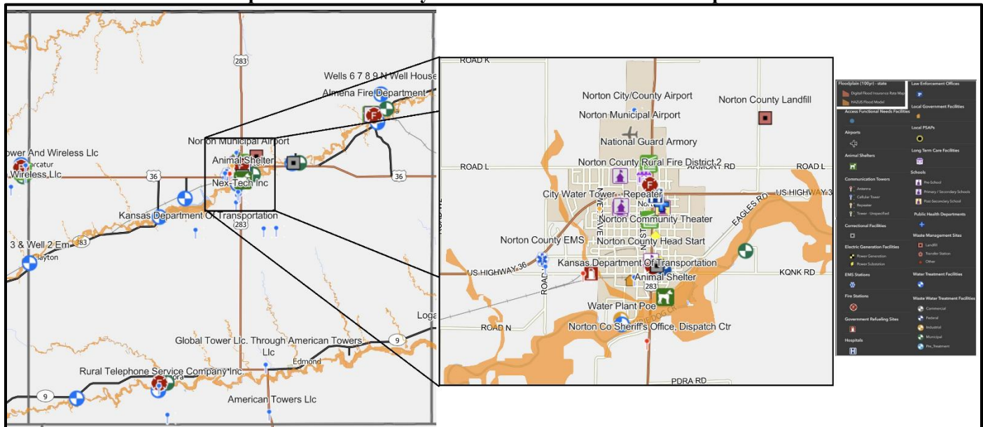
Map 76: Norton County Critical Infrastructure in Floodplains
