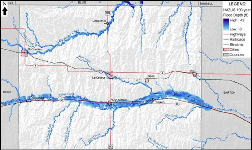
Map 64: Rush County Mapped Flood Areas
